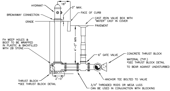
FIRE HYDRANT CONNECTION/LOCATION DETAIL
